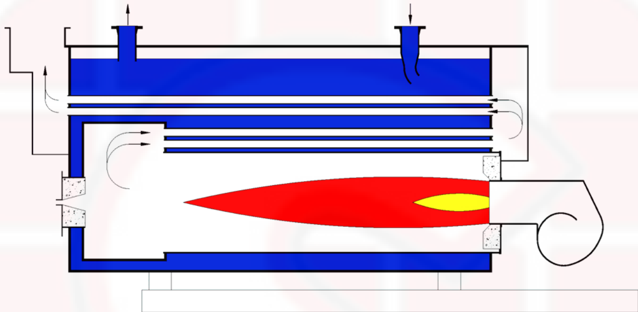
Graphic Depiction of 3-Pass Wetback Water Pass Configuration
