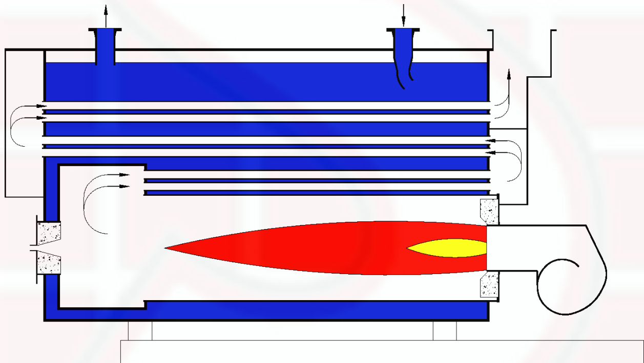
Graphic Depiction of 4-Pass Wetback Water Pass Configuration
