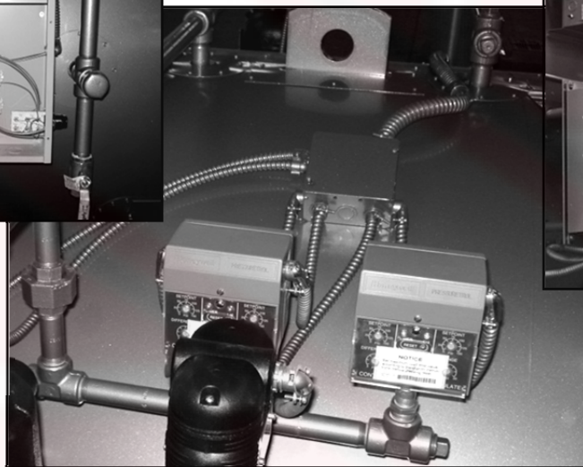
Example 4 x 4 junction box Figure 31b
