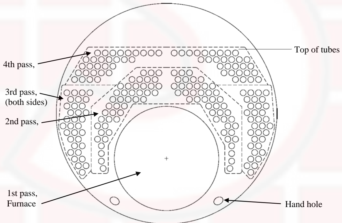
Example tube sheet: Figure 6
