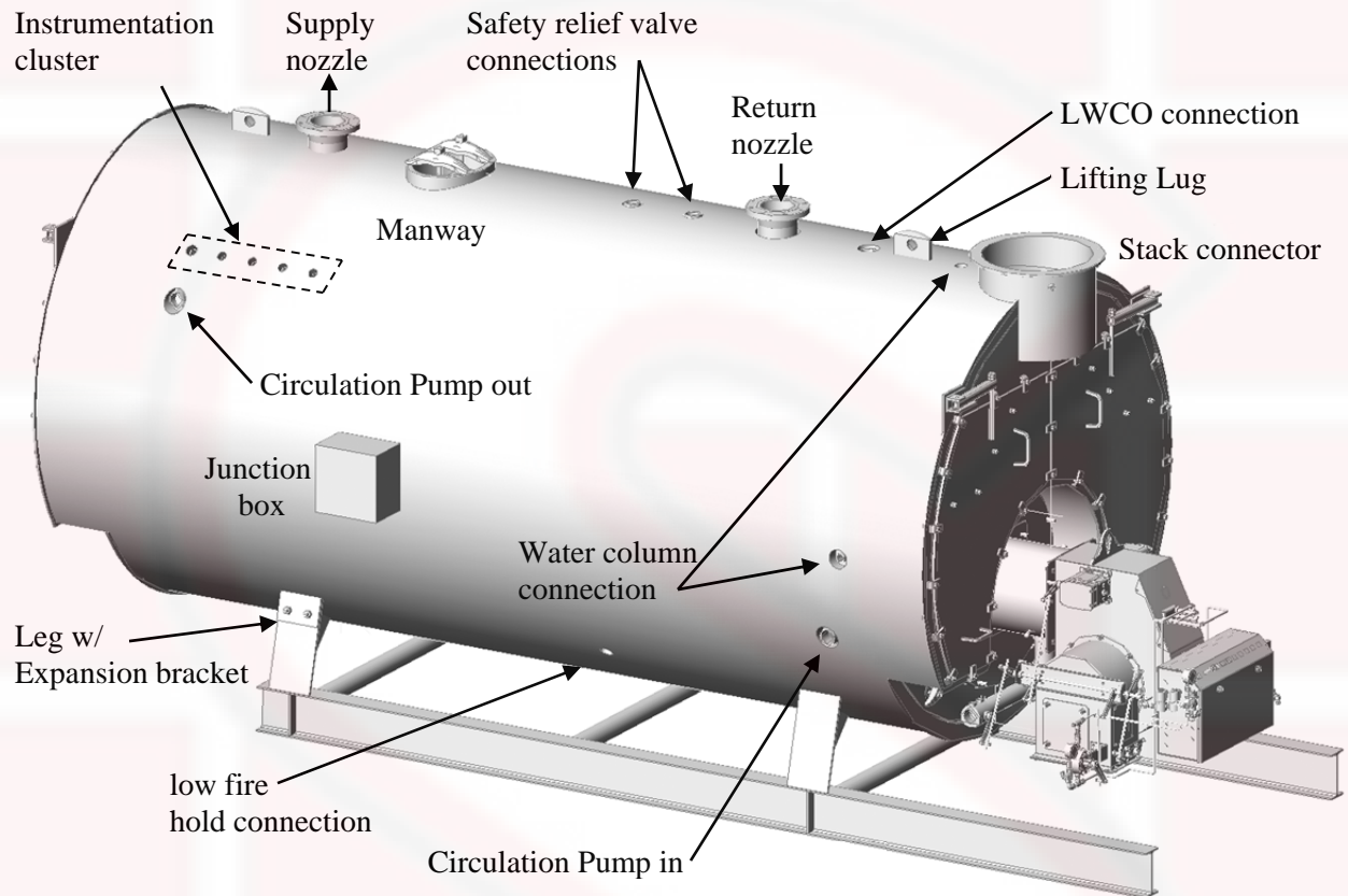
Water Boiler WO/ trim: Figure 3
