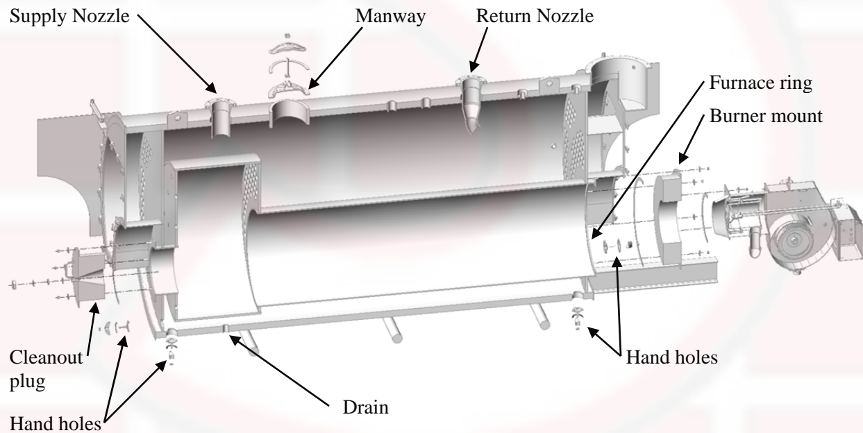
Water Boiler WO/ trim: Figure 3
